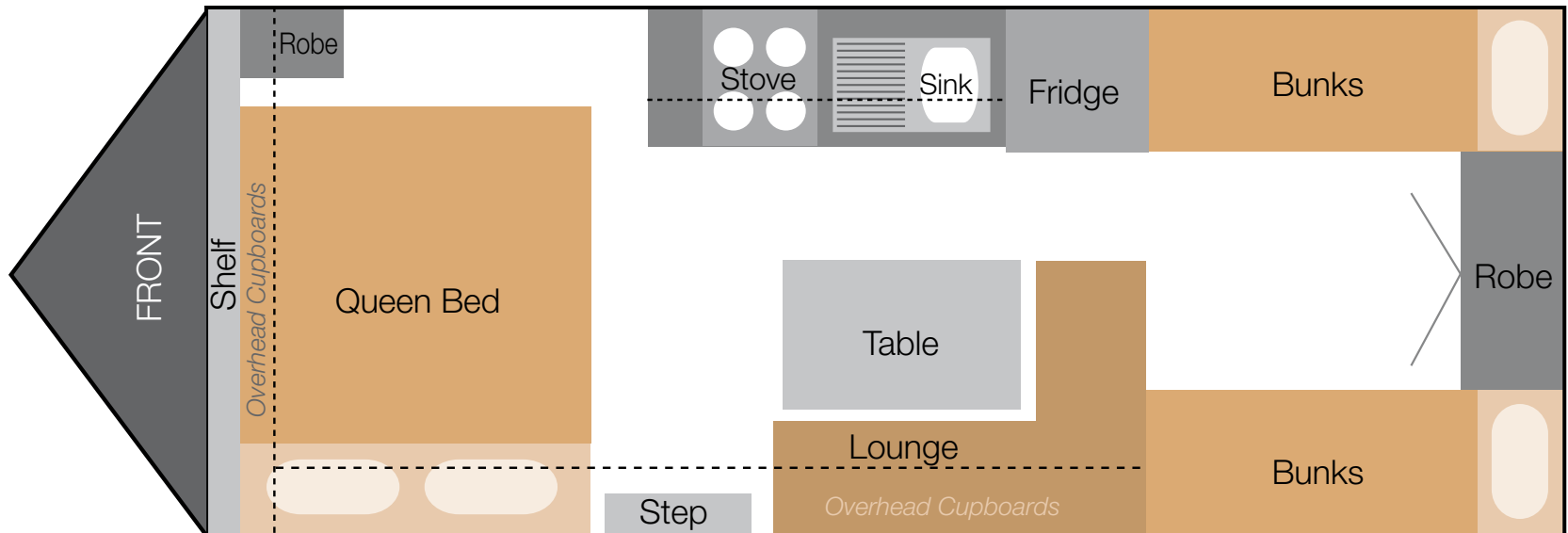
CB22 (19' - 6") INTERNAL
