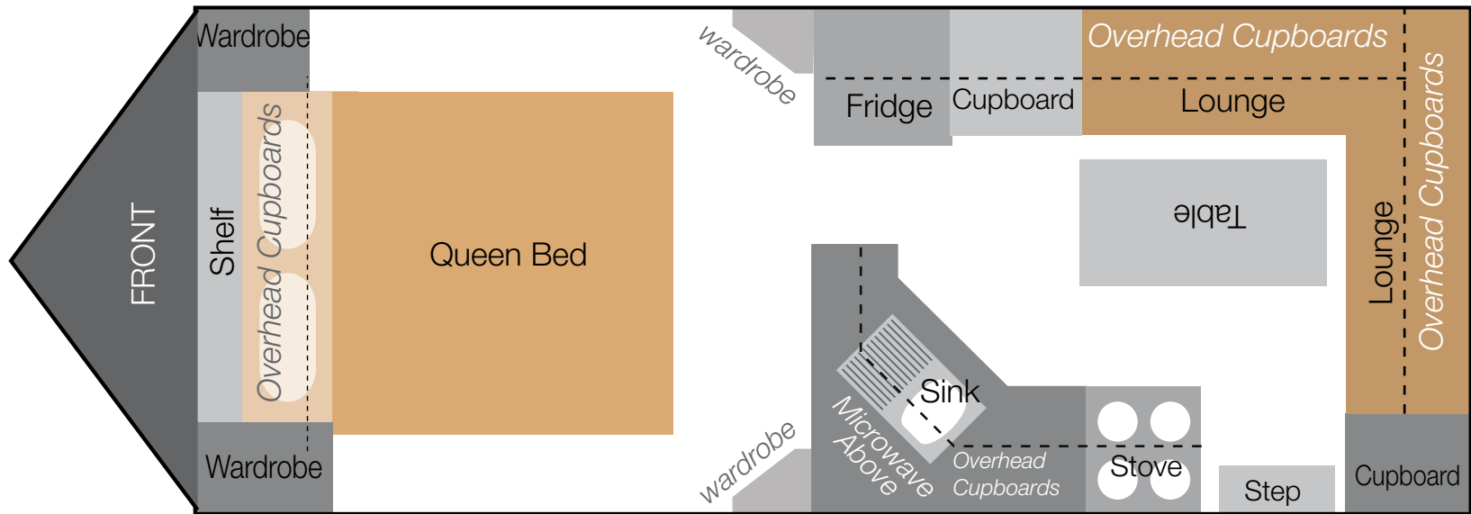
C04 (19' - 0") INTERNAL
