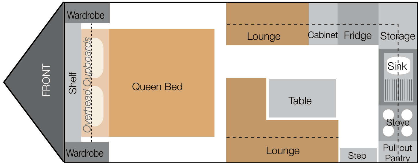
C03 (17' - 6'') INTERNAL
